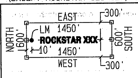
TYPICAL CLAIM DETAIL (NOT TO SCALE) (EXCEPT ROCKSTAR 123-126)
