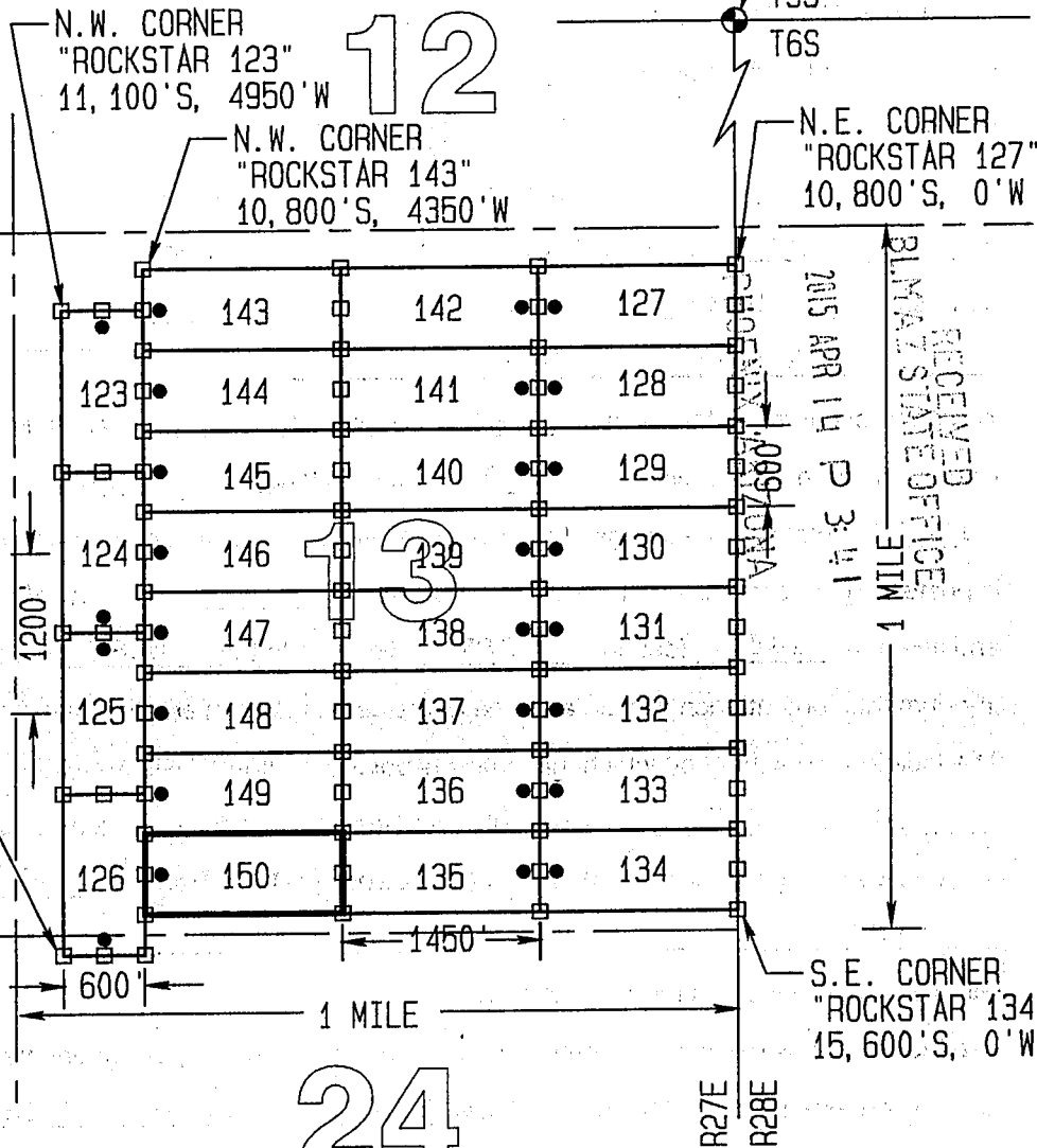
TYPICAL CLAIM DETAIL (NOT TO SCALE) (EXCEPT ROCKSTAR 123-126)
