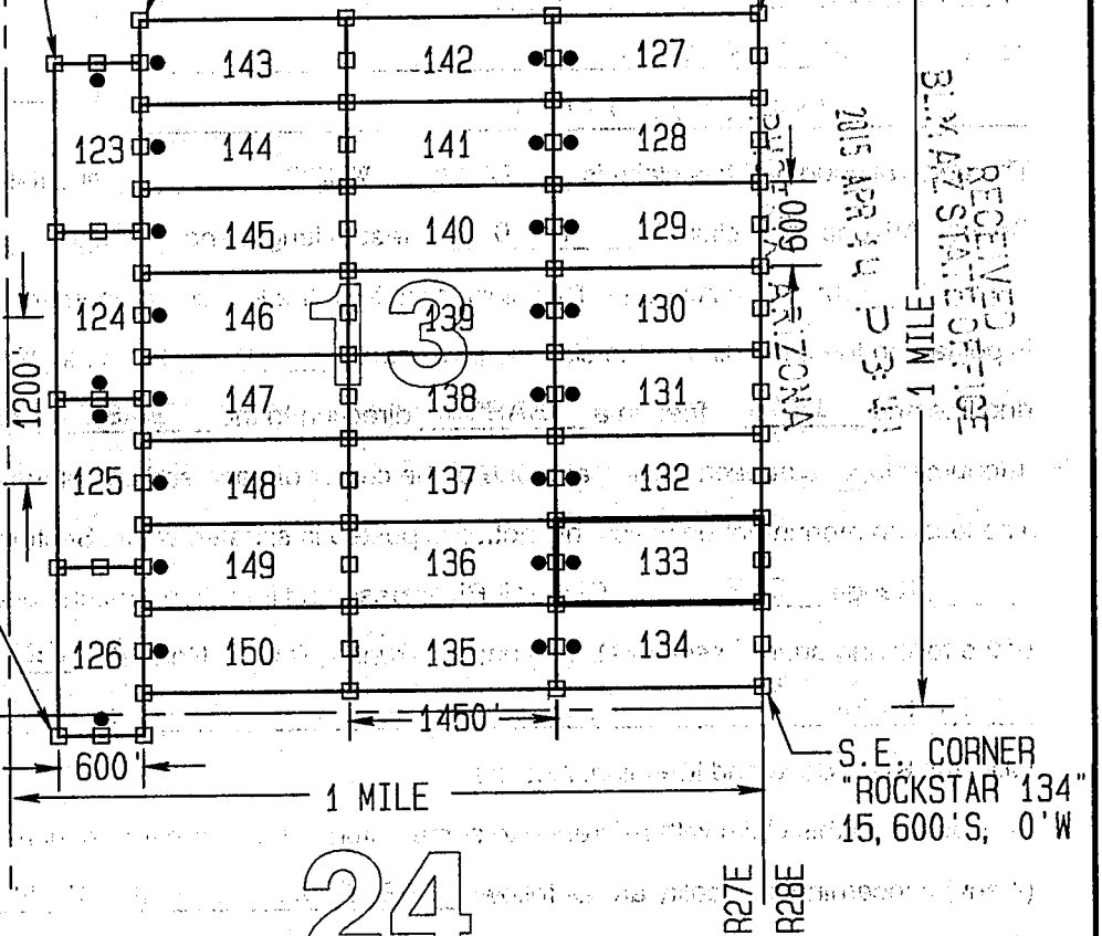
TYPICAL CLAIM DETAIL (NOT TO SCALE) (EXCEPT ROCKSTAR 123-126)
