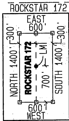
TYPICAL CLAIM DETAIL (NOT TO SCALE)
